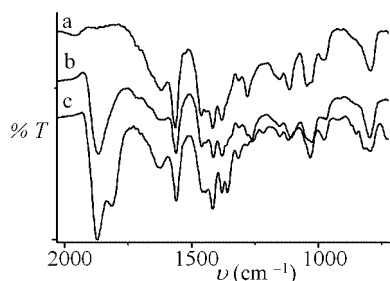
Figure 5. IR spectra of a) compound 3 , b) compound 3 with NO bubbled through and c) compound 6 .
