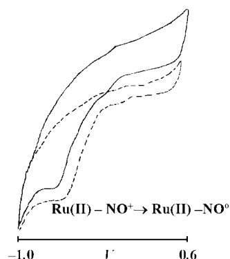
Figure 6. Cyclic voltammograms of complexes 5 (---) and ( 2 + NO) (—).
